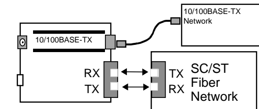
Fig. 3 Basic Network Connection
